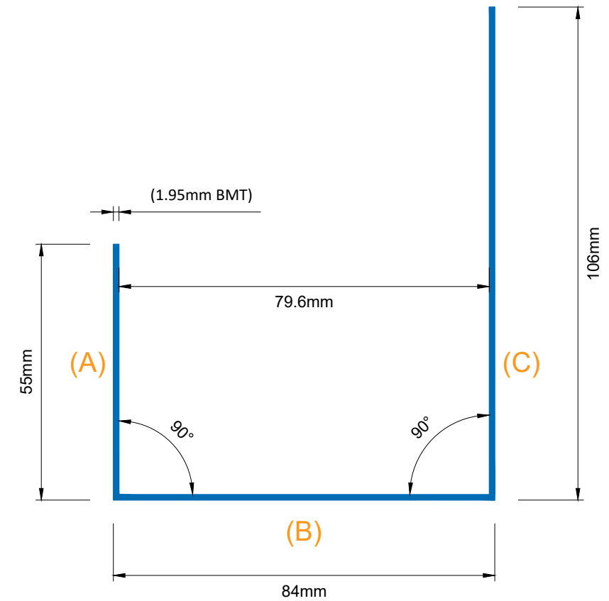
SPEEDPANEL® J-track 78mm 55/84/106 1.95mm BMT
