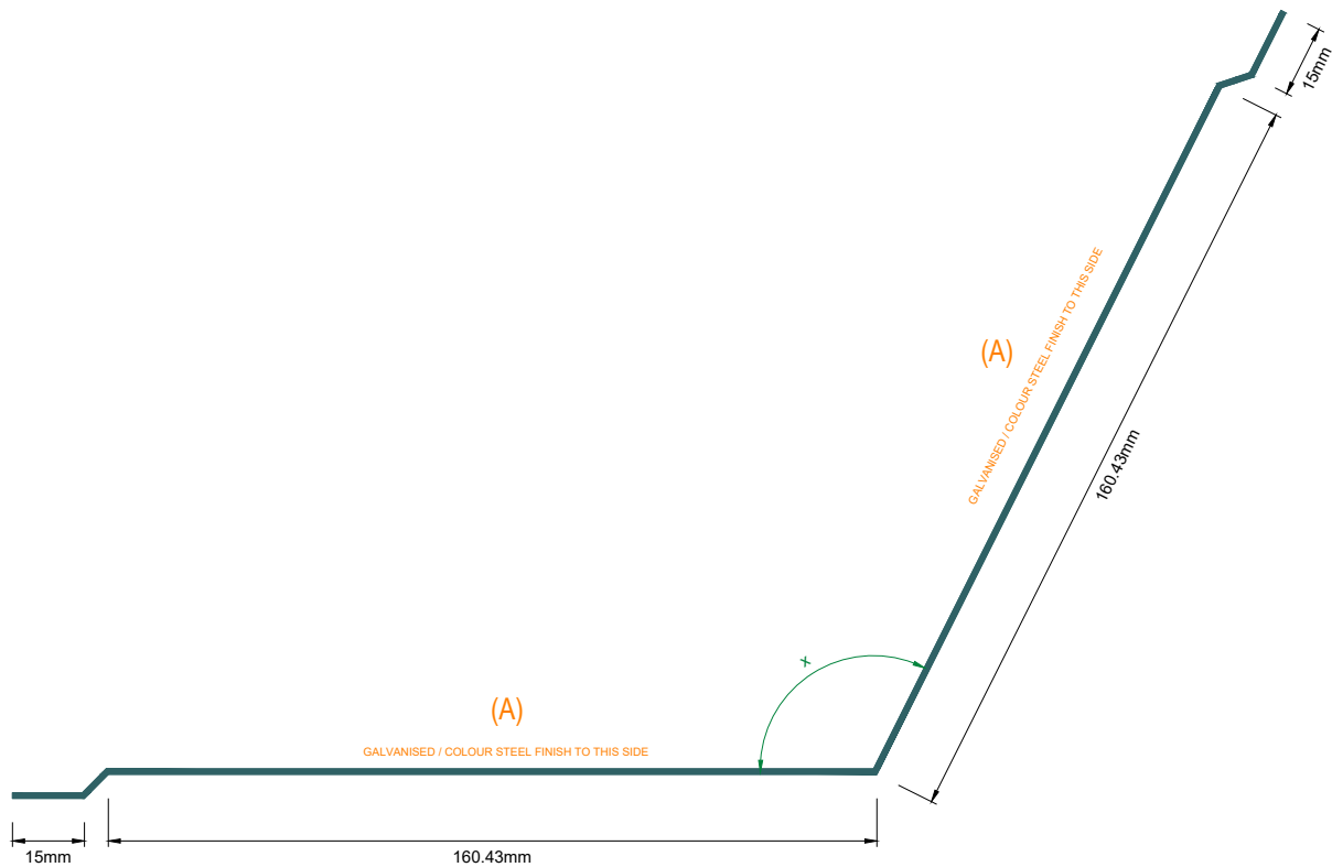
SPEEDPANEL® Internal Corner Flashing Obtuse 1.15mm BMT
