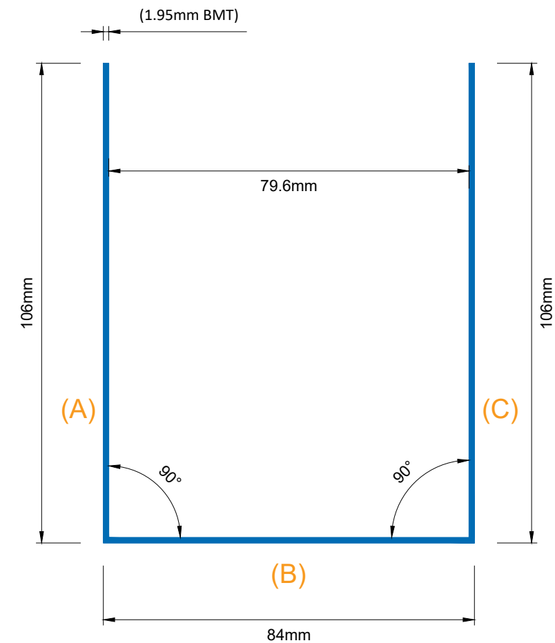
SPEEDPANEL® C-track 78mm 106/84/106 1.95mm BMT
