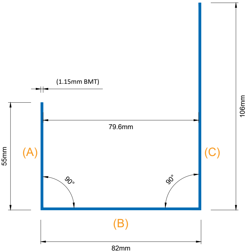
SPEEDPANEL® J-track 78mm 55/82/106 1.15mm BMT
