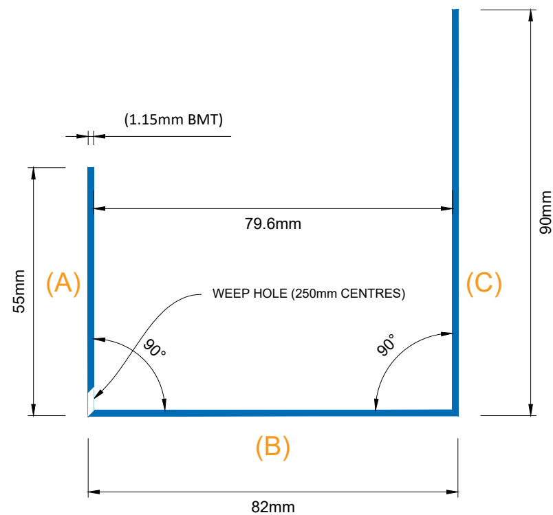
SPEEDPANEL® J-track 78mm 55/82/90 1.15mm BMT (Weep Holes)
