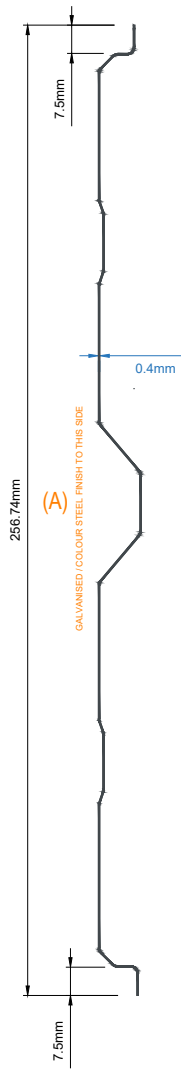
SPEEDPANEL® Flashing Cover Skin 0.4mm BMT
