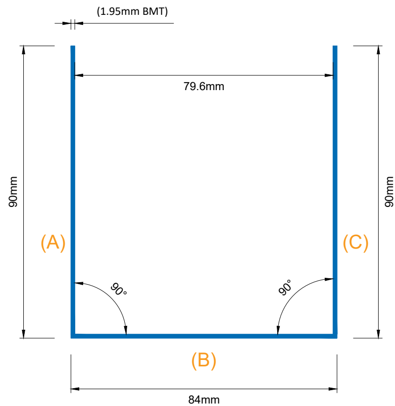
SPEEDPANEL® C-track 78mm 90/84/90 1.95mm BMT
