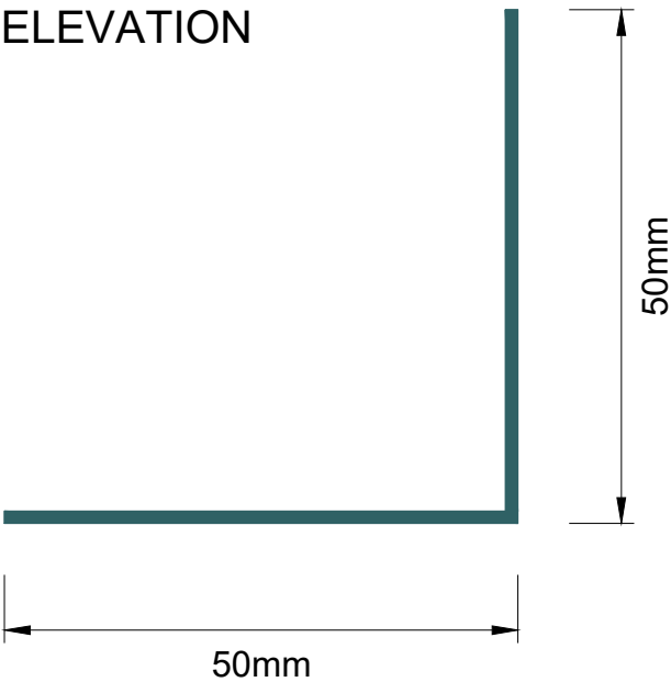
SPEEDPANEL® Angle Equal 50x50x1.15mm BMT
