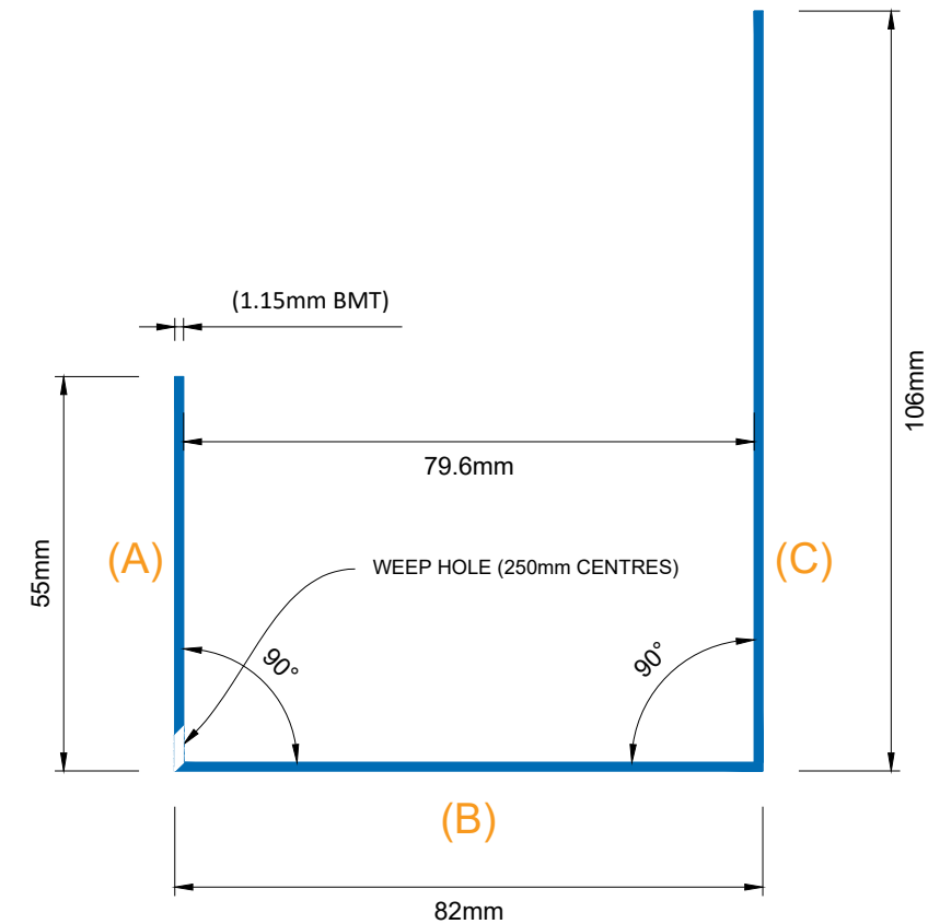
SPEEDPANEL® J-track 78mm 55/82/106 1.15mm BMT (Weep Holes)
