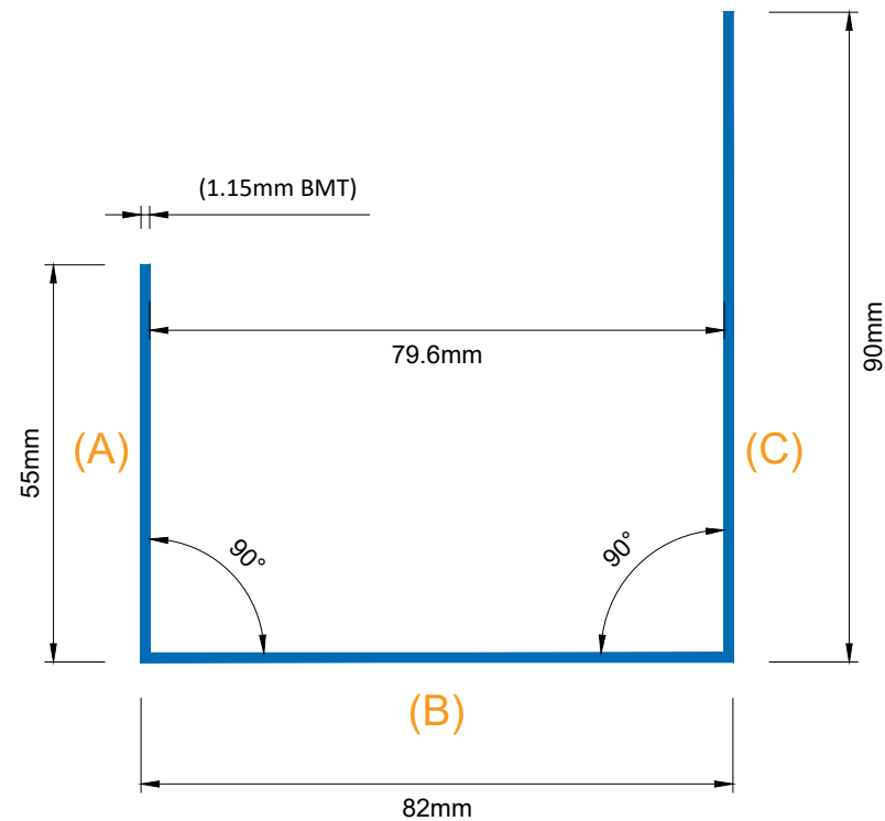
SPEEDPANEL® J-track 78mm 55/82/90 1.15mm BMT
