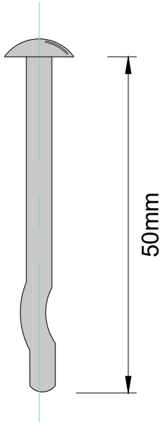
SPEEDPANEL® Mushroom Head Spikes M6.5 x 50mm
