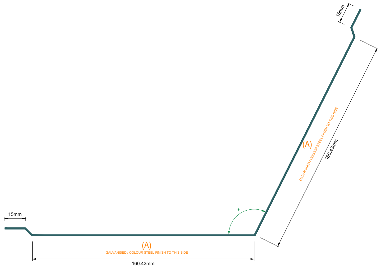
SPEEDPANEL® External Corner Flashing Obtuse 1.15mm BMT
