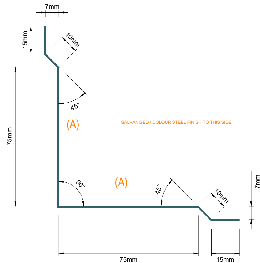
SPEEDPANEL® Internal Corner Flashing 90 Degree 0.7mm BMT
