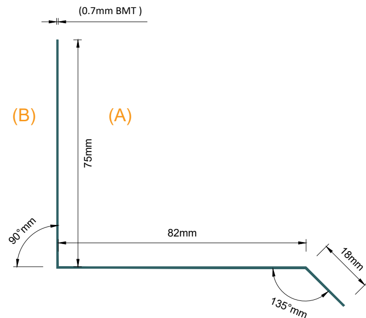
SPEEDPANEL® Flashing 78mm Z-Profile 0.7mm BMT
