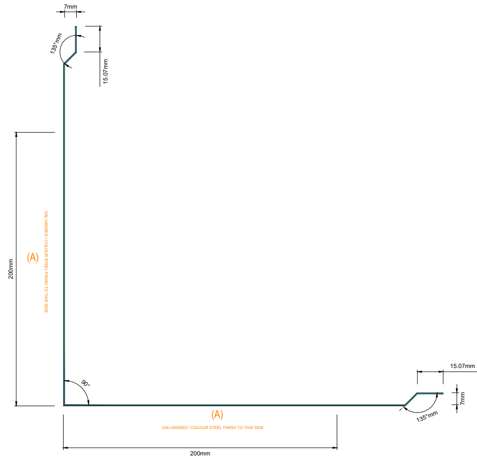
SPEEDPANEL® External Corner Flashing 90 Degree 0.7mm BMT
