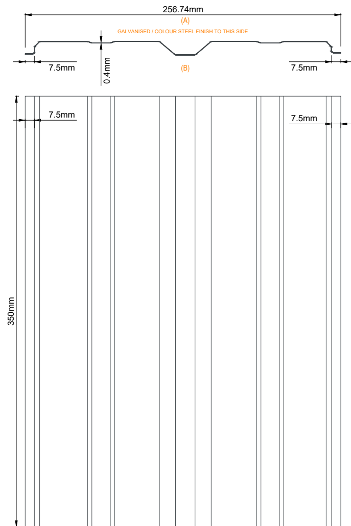
SPEEDPANEL® Flashing Cover Plate 0.4mm BMT 350mm Lengths
