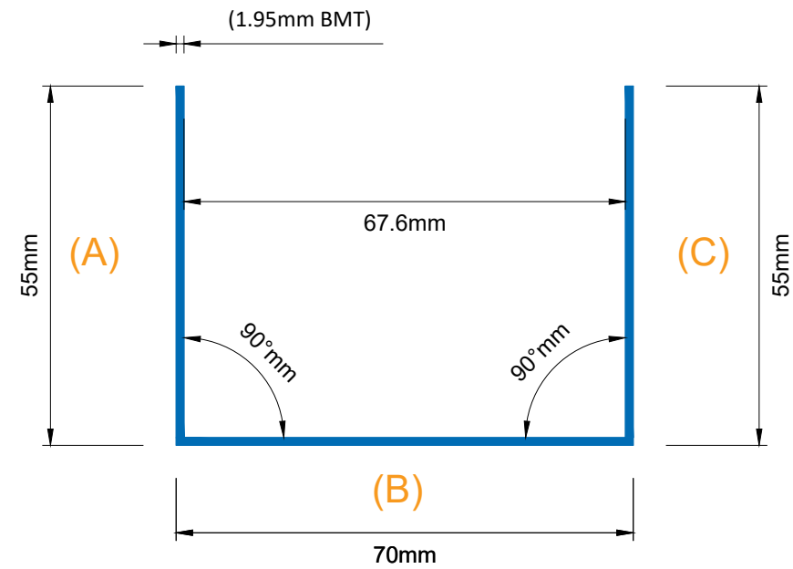
SPEEDPANEL® C-track 64mm 55/70/55 1.95mm BMT
