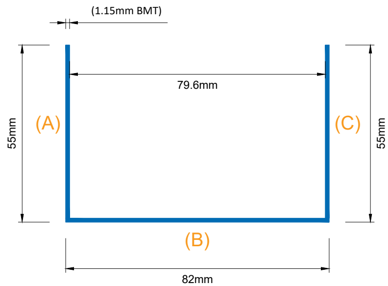
SPEEDPANEL® C-track 55/82/55 1.15mm BMT
