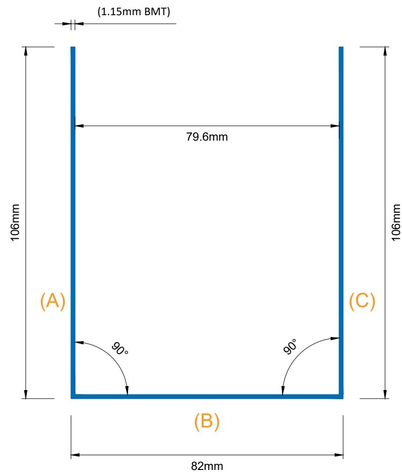
SPEEDPANEL® C-track 78mm 106/82/106 1.15mm BMT
