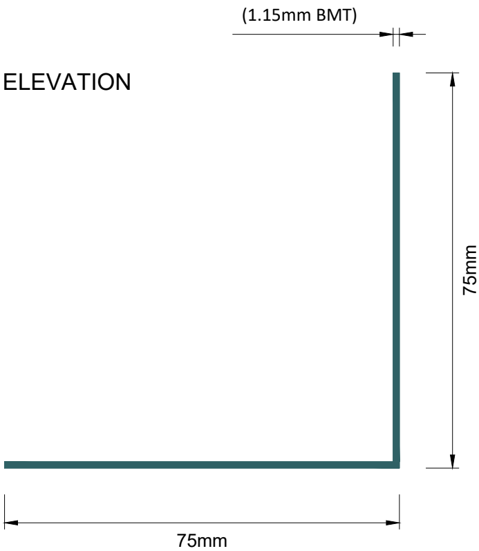
SPEEDPANEL® Angle Equal 75x75x1.15mm BMT
