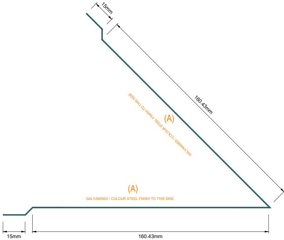
SPEEDPANEL® Internal Corner Flashing Acute 1.15mm BMT
