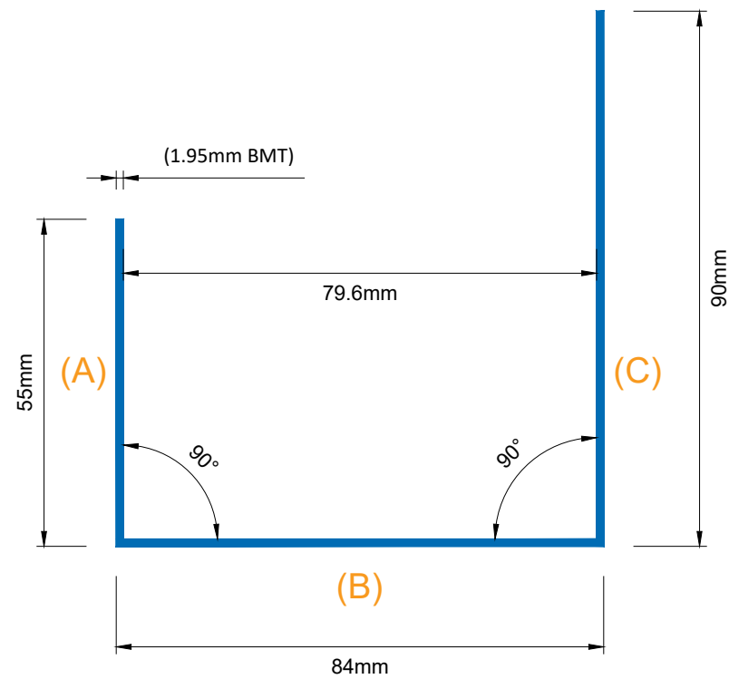
SPEEDPANEL® J-track 78mm 55/84/90 1.95mm BMT
