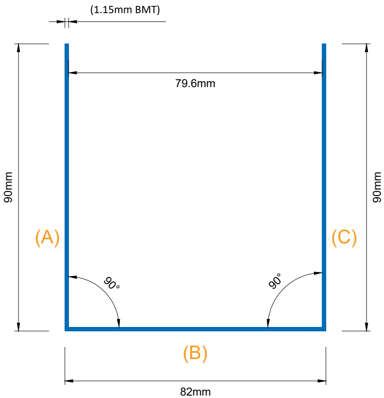
SPEEDPANEL® C-track 78mm 90/82/90 1.15mm BMT
