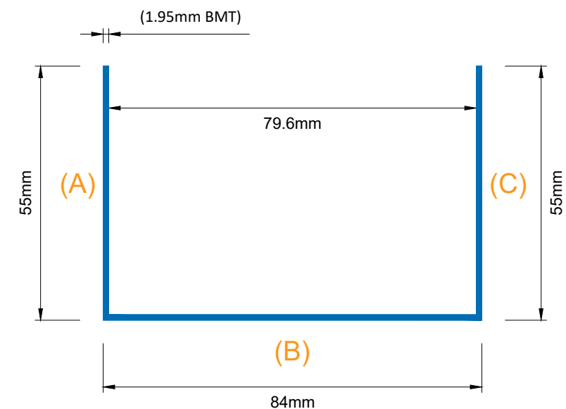
SPEEDPANEL® C-track 78mm 55/84/55 1.95mm BMT
