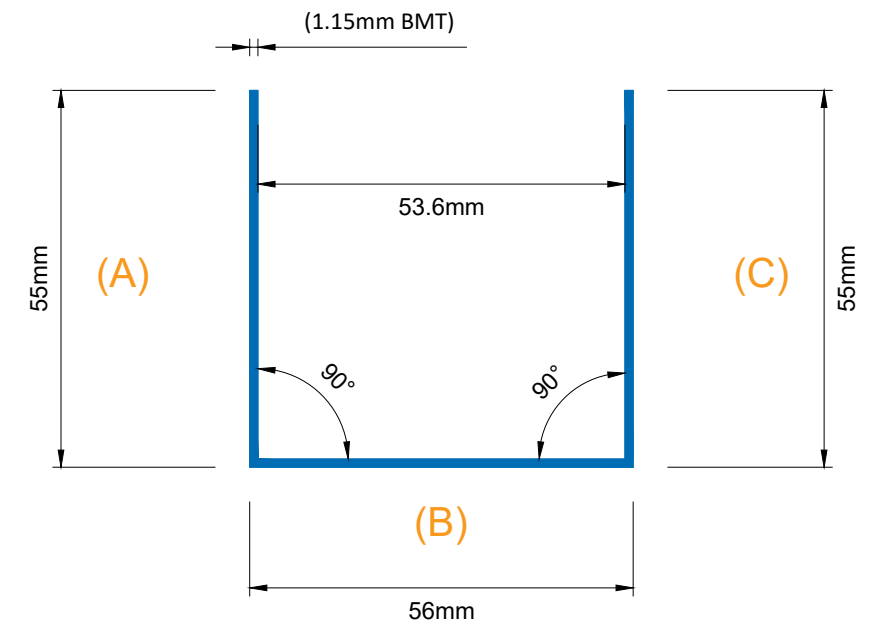
SPEEDPANEL® C-track 51mm 55/56/55 1.15mm BMT
