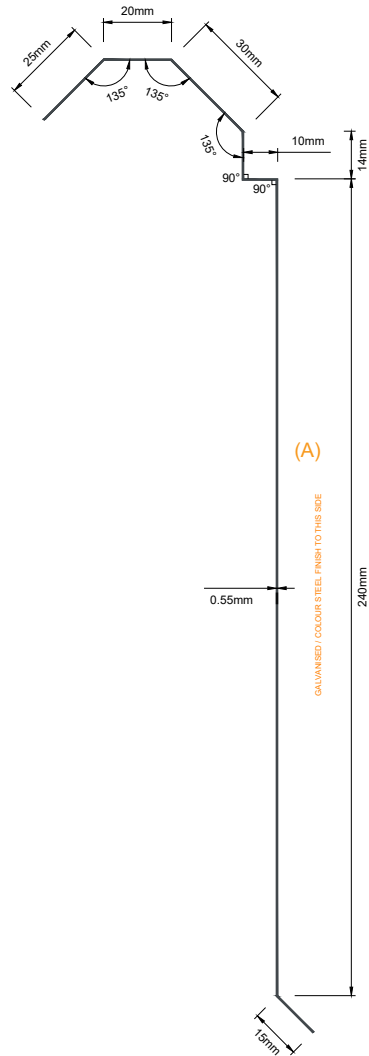
SPEEDPANEL® Flashing 78mm Cover External Joint Full 0.55mm BMT (Horizontal External Application)
